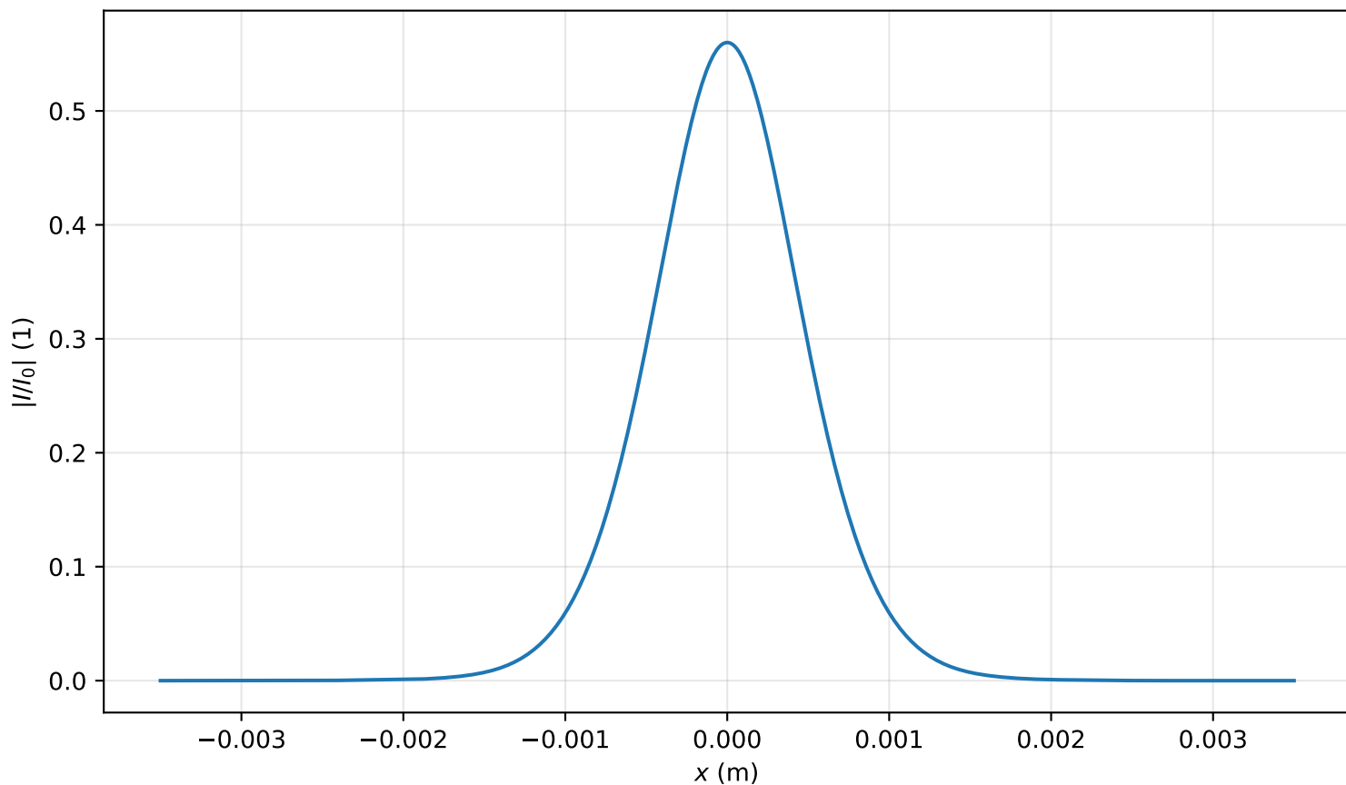
Intensity profile I(x, y = 0, z = 3.025m)/I_0 , P_{in}=0.5P_{cr} , artificial time
